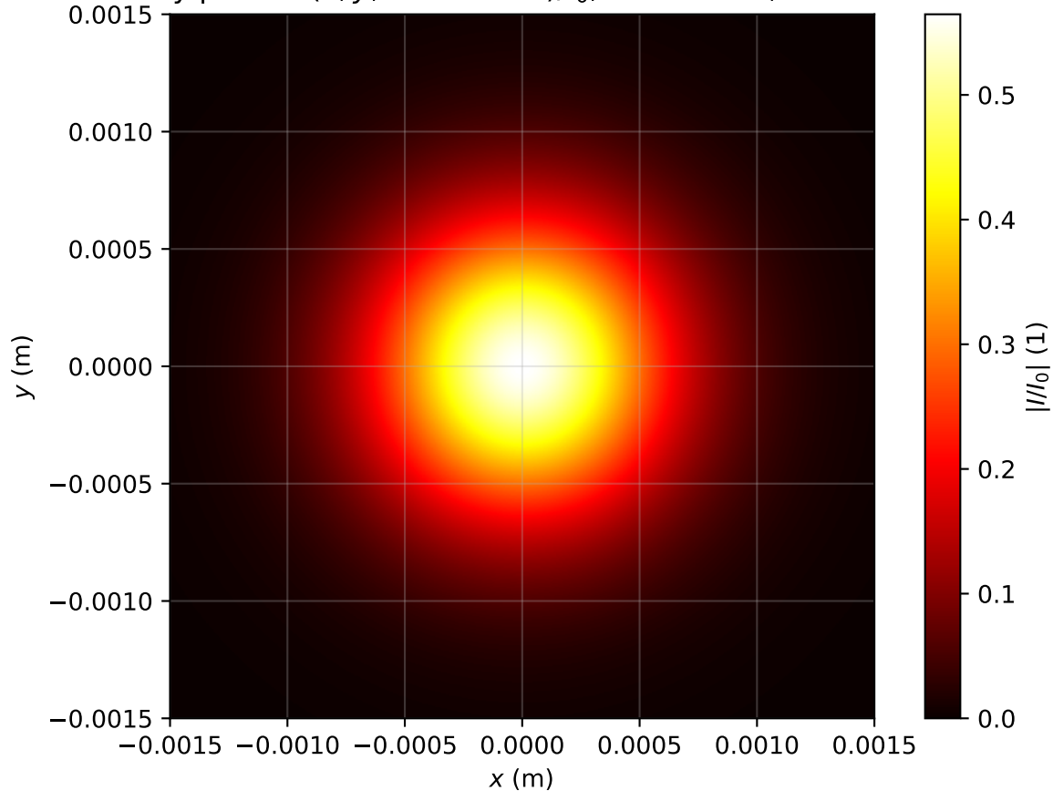
Intensity profile I(x, y, z = 2.627m)/I_0 , Pin=0.4Pcr, artificial time
